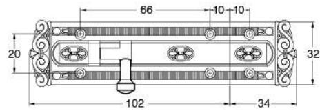
Dimension
